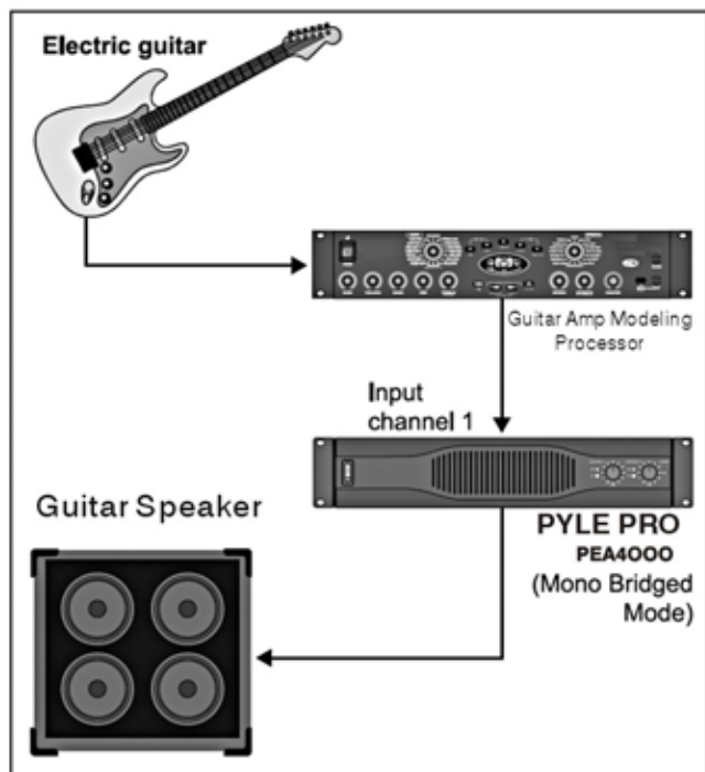
Fig .3.5: Mono-bridged mode
